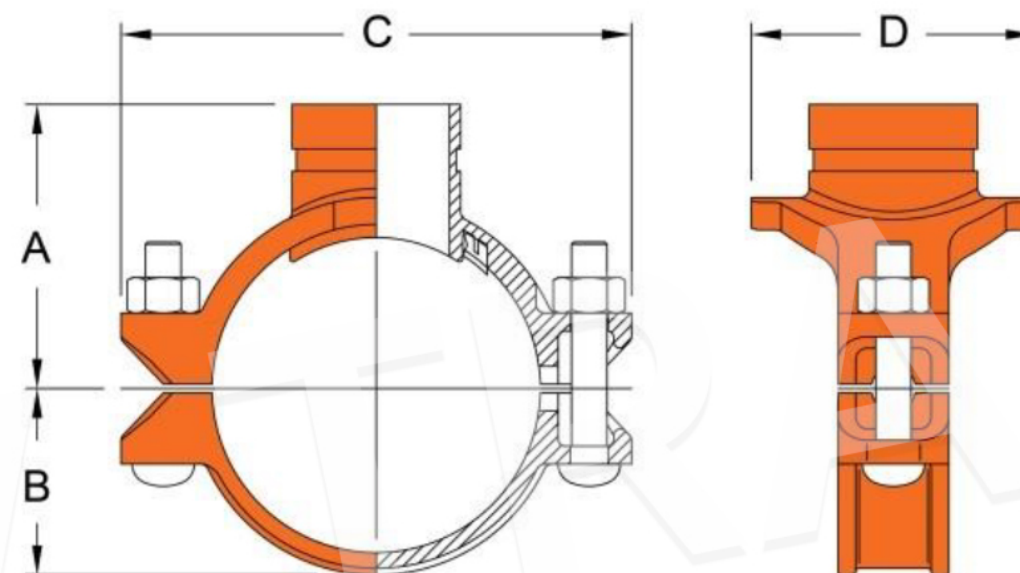
Model M22 Mechanical Tee, Grooved-End Outlet
